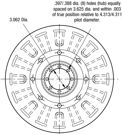
ARMATURE VIEW
